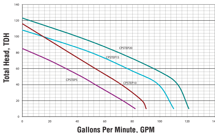
Champion Pump STEP Performance
